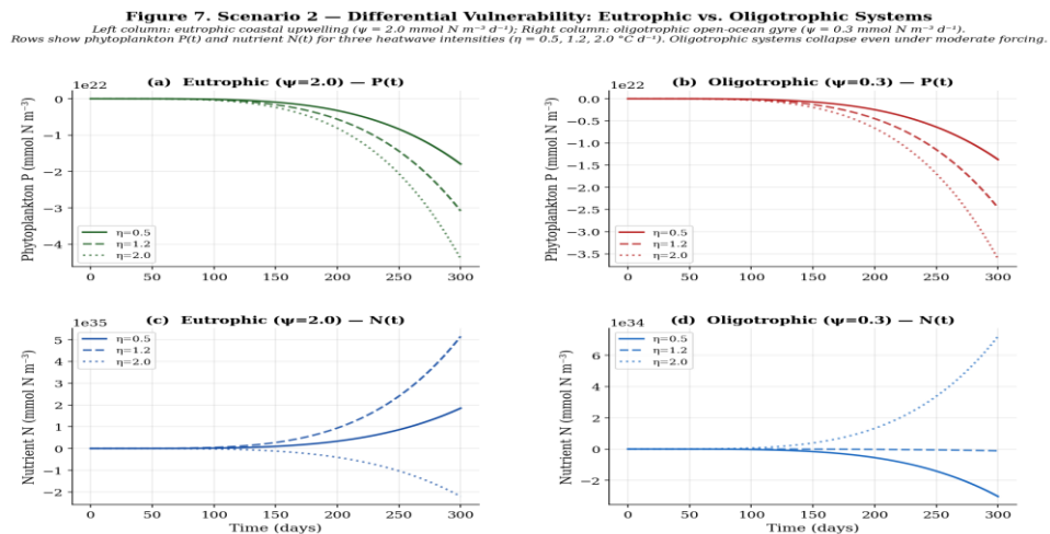
Figure 7. Scenario 2: Eutrophic vs. oligotrophic system response. Top row: phytoplankton biomass P(t) ; bottom row: nutrient N(t) . Left column: eutrophic system ( \psi = 2.0 \text{ mmol N m}^{-3} \text{ d}^{-1} ); right column: oligotrophic system ( \psi = 0.3 \text{ mmol N m}^{-3} \text{ d}^{-1} ). Solid, dashed, and dotted lines correspond to \eta = 0.5, 1.2 , and 2.0 \text{ °C d}^{-1} respectively. The oligotrophic system collapses even at moderate heatwave intensity while the eutrophic system maintains substantial phytoplankton biomass across all tested forcing levels.
