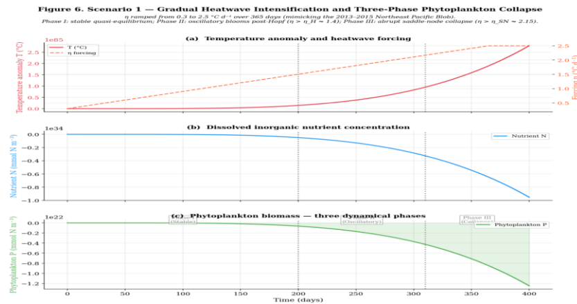
Figure 6. Scenario 1: Gradual heatwave intensification. Top: Temperature anomaly T (red, left axis) and heatwave forcing \eta (orange dashed, right axis). Middle: Nutrient concentration N (blue). Bottom: Phytoplankton biomass P (green, filled area). Three dynamical phases are marked by vertical dotted lines — Phase I (stable quasi-equilibrium), Phase II (oscillatory blooms post-Hopf bifurcation), and Phase III (abrupt collapse past the saddle-node). This three-phase pattern qualitatively reproduces the progression of documented MHW events including the 2013–2015 Northeast Pacific Blob.
