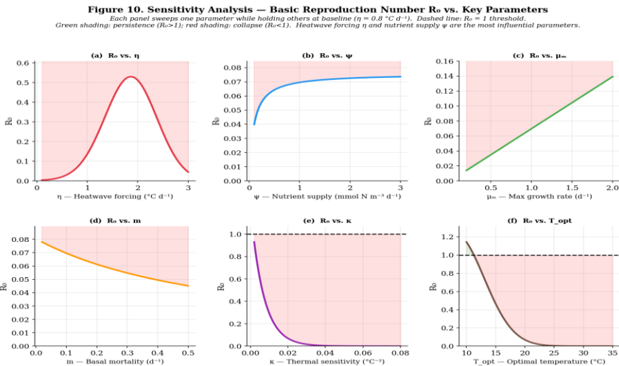
Figure 10. Sensitivity analysis of the basic reproduction number R_0 to six key model parameters ( \eta : forcing intensity; \psi : nutrient supply; \mu_m : max growth rate; m : mortality; \kappa : thermal sensitivity; T_{opt} : optimal temperature). Dashed line marks the R_0 = 1 threshold; green and red shading indicate persistence and collapse territories respectively. Parameters with the steepest R_0 slopes represent the greatest potential levers for ecosystem management or the greatest sources of model uncertainty. Nutrient supply \psi and heatwave forcing \eta emerge as the most influential parameters.
