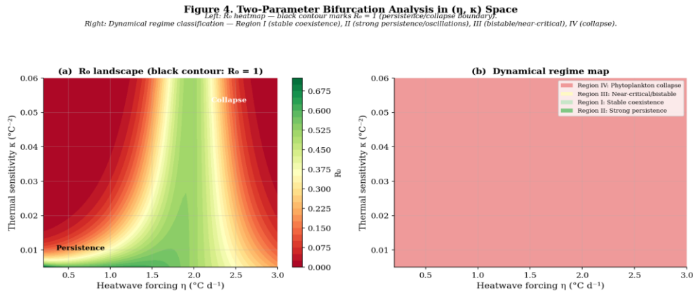
Figure 4. Two-parameter bifurcation analysis in (\eta, \kappa) space. Left: R_0 landscape as a heatmap, with the black contour marking R_0 = 1 . Warm colors (red) indicate collapse territory; cool colors (green) indicate phytoplankton persistence. Right: Classification of dynamical regimes — pale red (Region IV: collapse), yellow (Region III: near-critical/bistable), light green (Region I: stable coexistence), and dark green (Region II: strong persistence/oscillations). Species with higher thermal sensitivity (larger \kappa ) collapse at substantially lower heatwave intensities.
