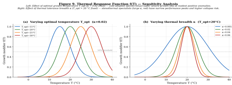
Figure 9. Thermal response function sensitivity analysis. Left: Effect of optimal growth temperature T_{opt} ( \kappa = 0.02 fixed) — species with low T_{opt} (e.g., cold-adapted diatoms, blue) experience severe growth suppression at modest positive anomalies, while warm-adapted species (red) may initially benefit from warming. Right: Effect of thermal tolerance breadth \kappa ( T_{opt} = 20^{\circ}\text{C} fixed) — stenothermal species (large \kappa , red) show sharp growth declines on either side of the optimum, while eurythermal species (small \kappa , blue) maintain substantial growth rates over a wide temperature range. The 50% growth-rate threshold (grey dotted line) is crossed at progressively smaller temperature anomalies as \kappa increases.
